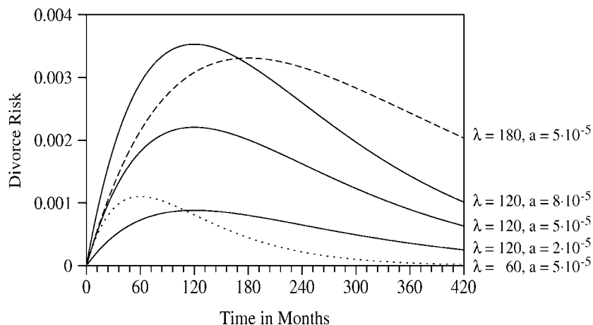
Figure 1: The sickle model of the divorce risk function. Hazard rate curves for different values of the parameterands \lambda and a .
